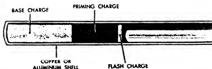
NON-ELECTRIC BLASTING CAP
